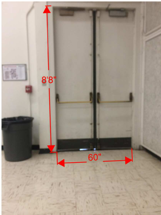
Existing Door and Frame D-1 and D-2 Similar.
