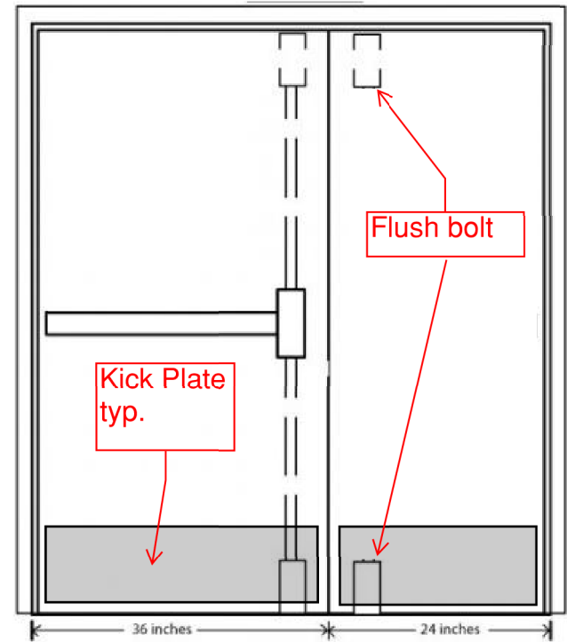
New Door Configuration, uneven leaf, no center mullion doors and frame.
